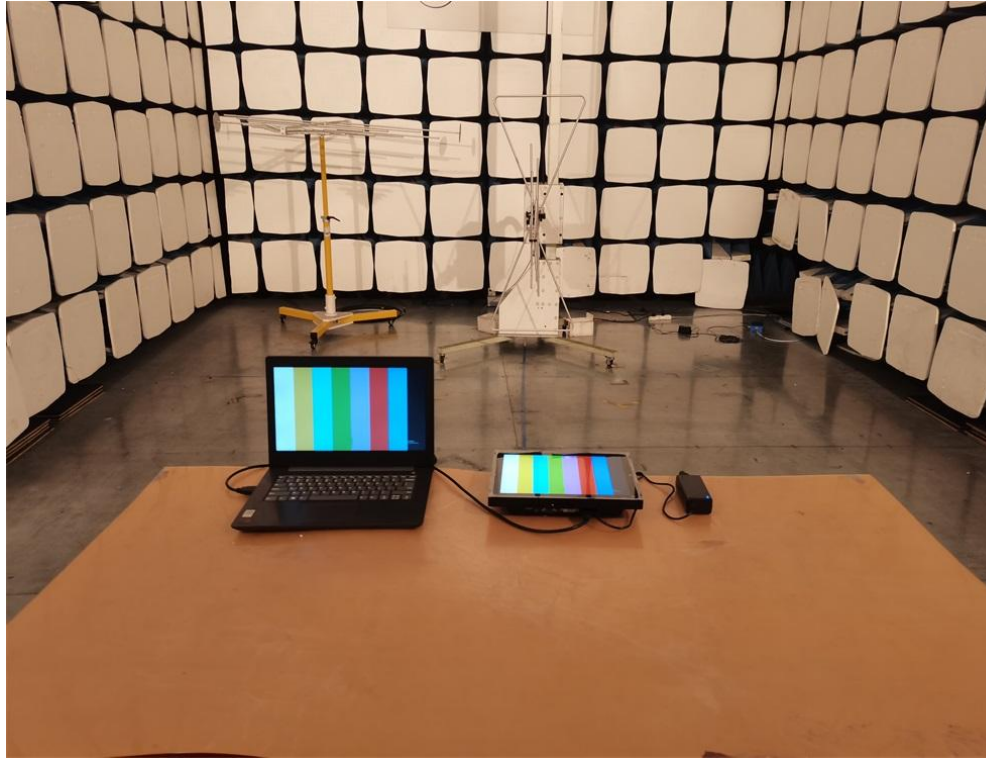
Radiated Emission
